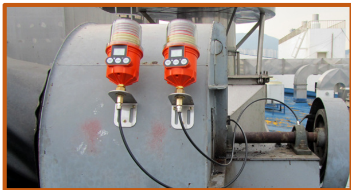
Fan bearing – remote mount 125cc Pulsarlube Customer supply tube and fittings (Order Codes 91-GL125 & 41-LBK-1-000-O-BRA)
